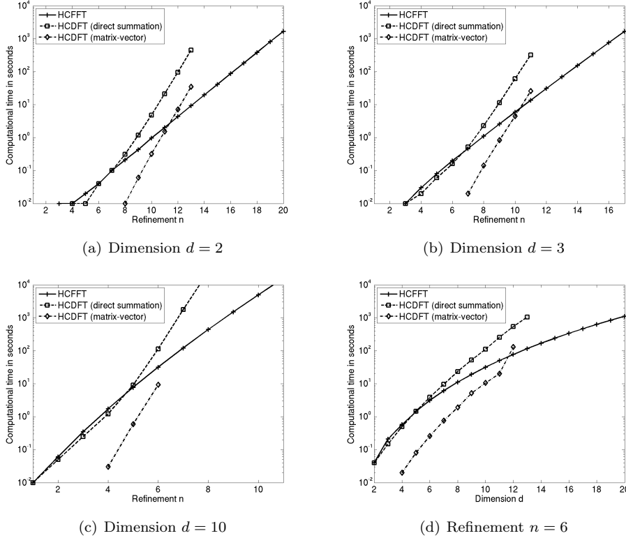
FIGURE 5.1. Computational time for the HCDFT and HCFFT with respect to the refinement n and the dimension d .
