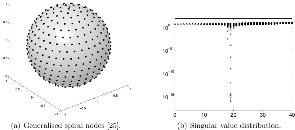
Figure 1 Distribution of the singular values of the spherical Fourier matrix \mathbf{Y} \in \mathbb{C}^{M \times (N+1)^2} with respect to the polynomial degrees N = 0, \dots, 40 for M = 400 generalised spiral nodes.
