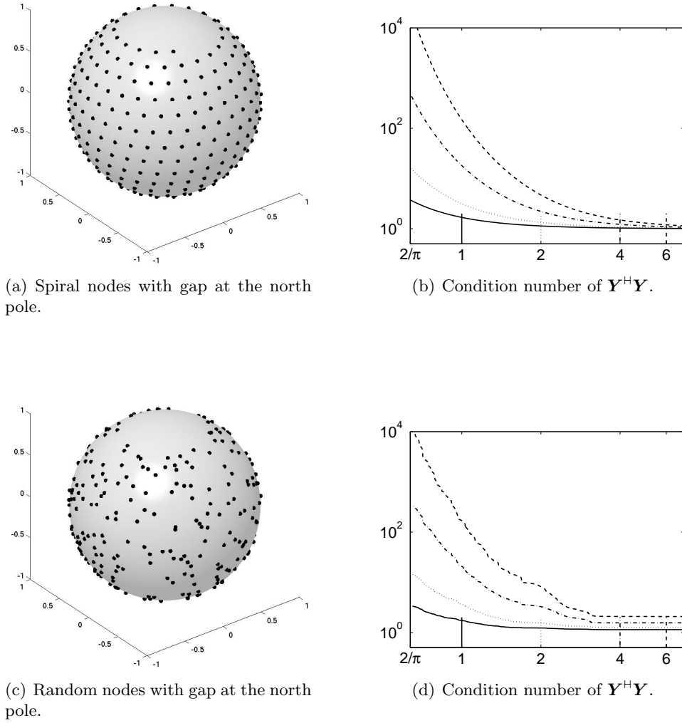
Figure 4 Condition number \text{cond}(\mathbf{Y}^H \mathbf{Y}) , \mathbf{Y} \in \mathbb{C}^{M \times (N+1)^2} , with respect to the approximate inverse mesh norm \delta_{\mathcal{X}}^{-1} \in [2/\pi, \dots, 7) , i.e., 200 \leq M \leq 400 . The polynomial degree is N = 1 (solid), N = 2 (dotted), N = 4 (dash-dot), and N = 6 (dashed).
