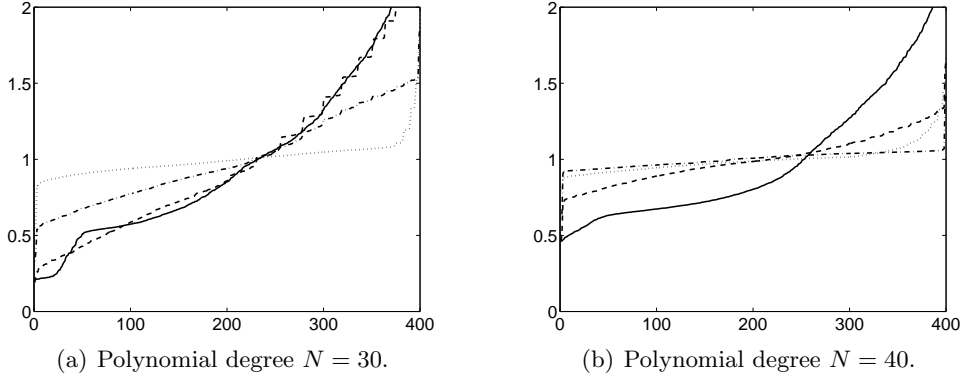
Figure 5 Eigenvalue distribution of the matrix \mathbf{K} = \mathbf{Y}\hat{\mathbf{W}}\mathbf{Y}^H \in \mathbb{C}^{M \times M} for weighting matrices obtained from the sampled B-spline of order \beta = 1 (solid), \beta = 2 (dotted), \beta = 3 (dash-dot), and \beta = 4 (dashed).
