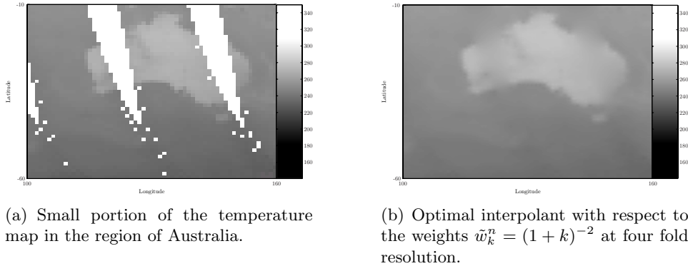
Figure 6 Optimal interpolation using a small portion of the temperature map.
