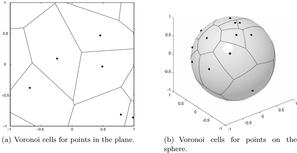
Figure 2 Voronoi cells in the plane and on the sphere.
