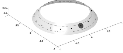
Figure 3 The set S_{\mathcal{X},q,m} , the ring S_{q,m} (dashed), the larger ring \tilde{S}_{q,m} , and a spherical cap of colatitude q/2 centred at one node for generalised spiral nodes.
